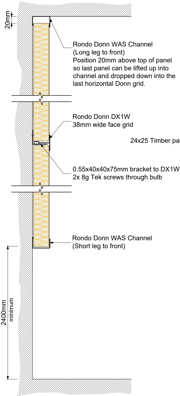
T-Grid Option
