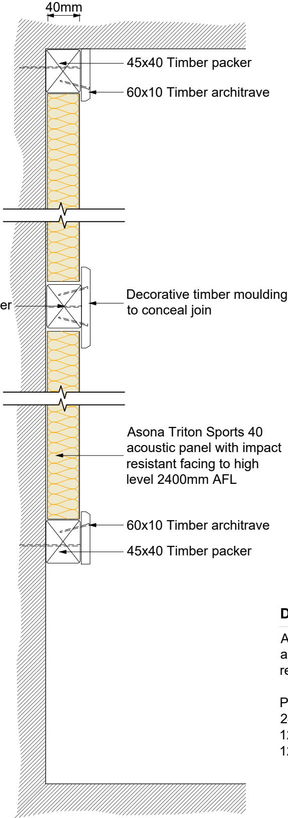
Timber Option
