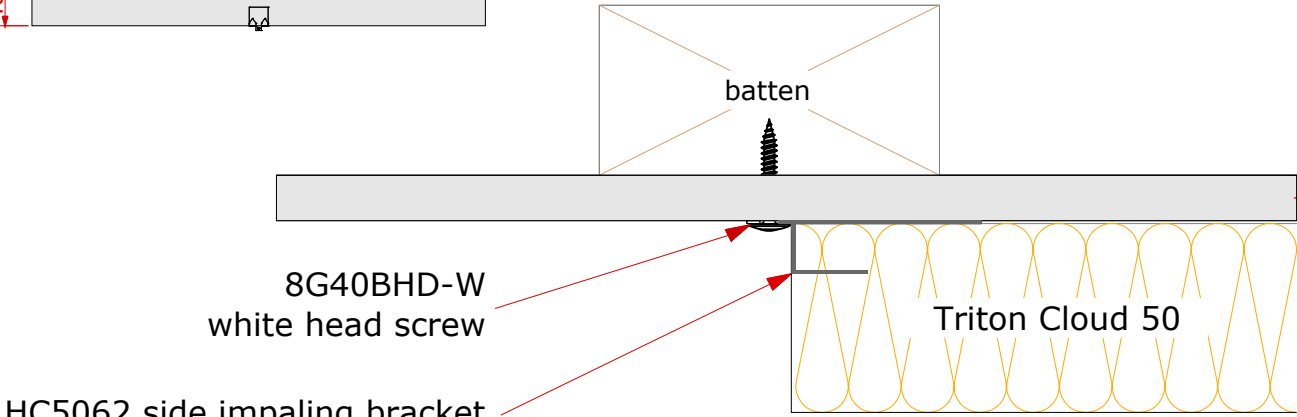
Fixing Option 1
