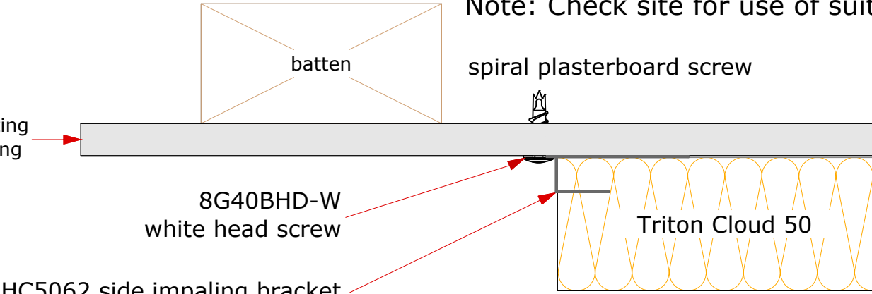
Fixing Option 2
