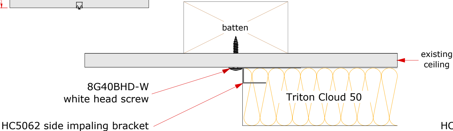
Fixing Option 1
