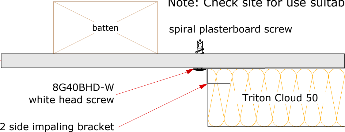
Fixing Option 2
