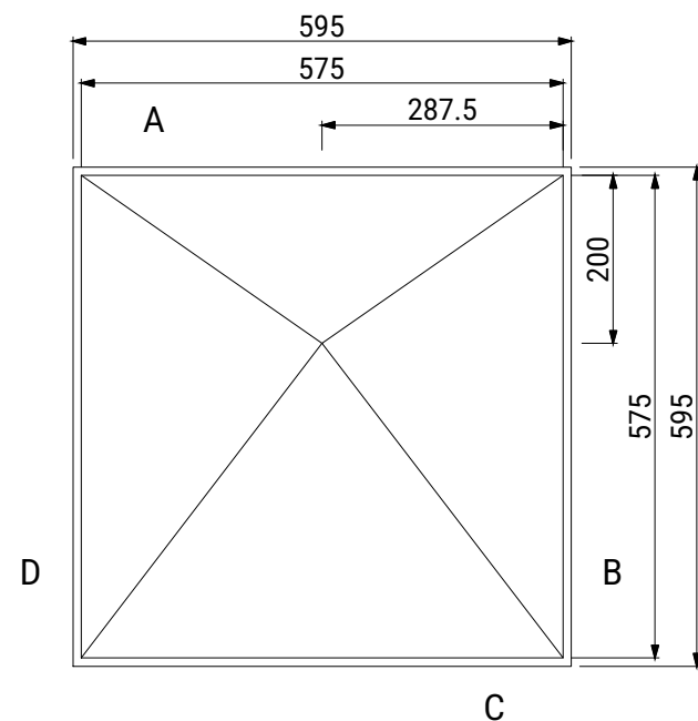
Pyramid 3D Dimensions
