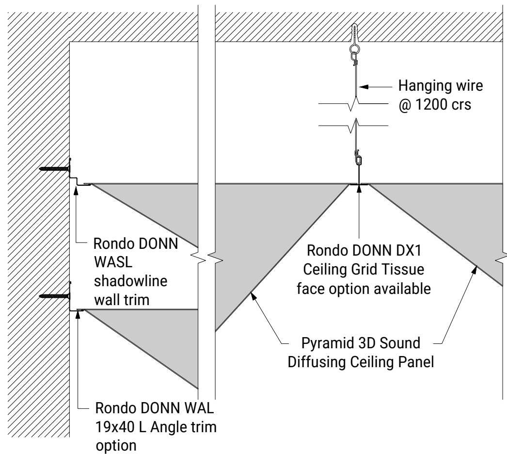
Suspended Fixing Detail
