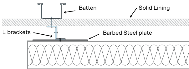
Detail: Barbed Steel Plate for "L to L" direct fix.
