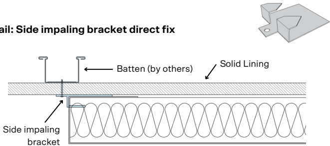
Detail: Side impaling bracket direct fix to batten
