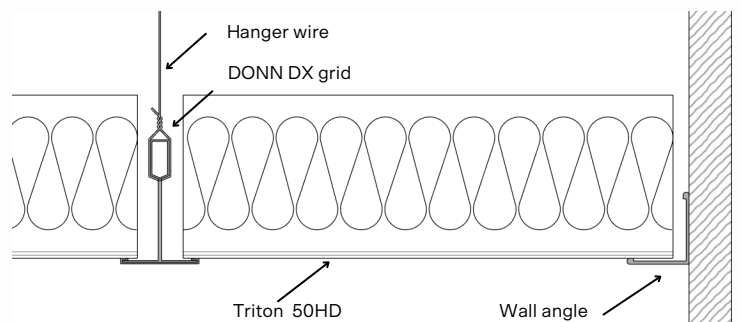
Detail: Triton 50HD ceiling tile suspended on Rondo Donn DX Grid
