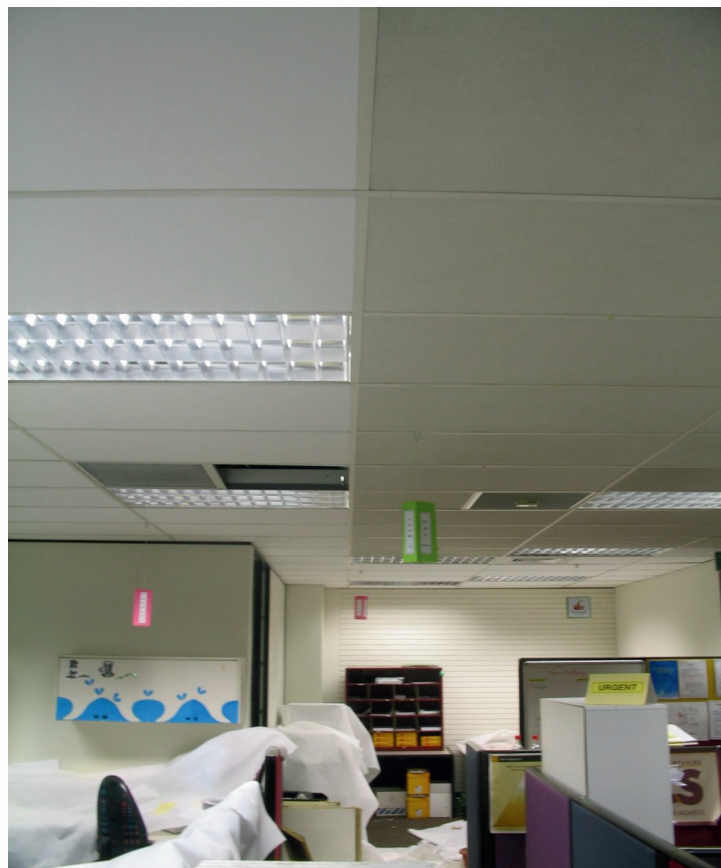
Above: 1/2 completed ceiling, new Sonatex finish applied top left with 12 year old rockwool ceiling panels top right
