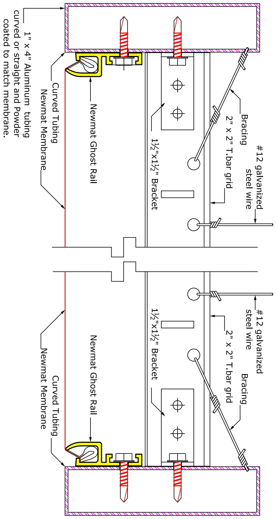
Newmat Free Floating Edge Detail Art-24
