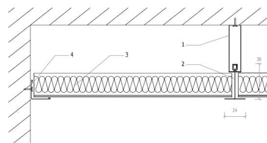
Top: Otara library, 1200 x 1200 mm Triton 25 composite soft fibre absorber panels on T24 grid
