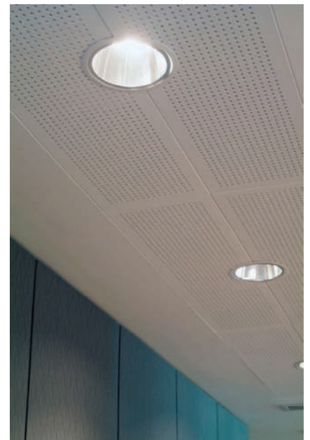
Left and top: Waiting Room, 60 mm thick Asona Sound Soft stretch fabric sound absorber wall panels with 10 mm negative for quiet comfort. Right: Danoline Tectopanel 1200 x 300 x 13mm perforated gypsum acoustic panel detail set in flush stopped plasterboard ceiling
