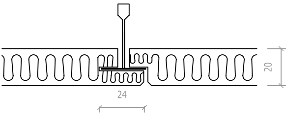
T24 Concealed edge (2 side shiplap, 2 sides bevel) Scale 1:2
